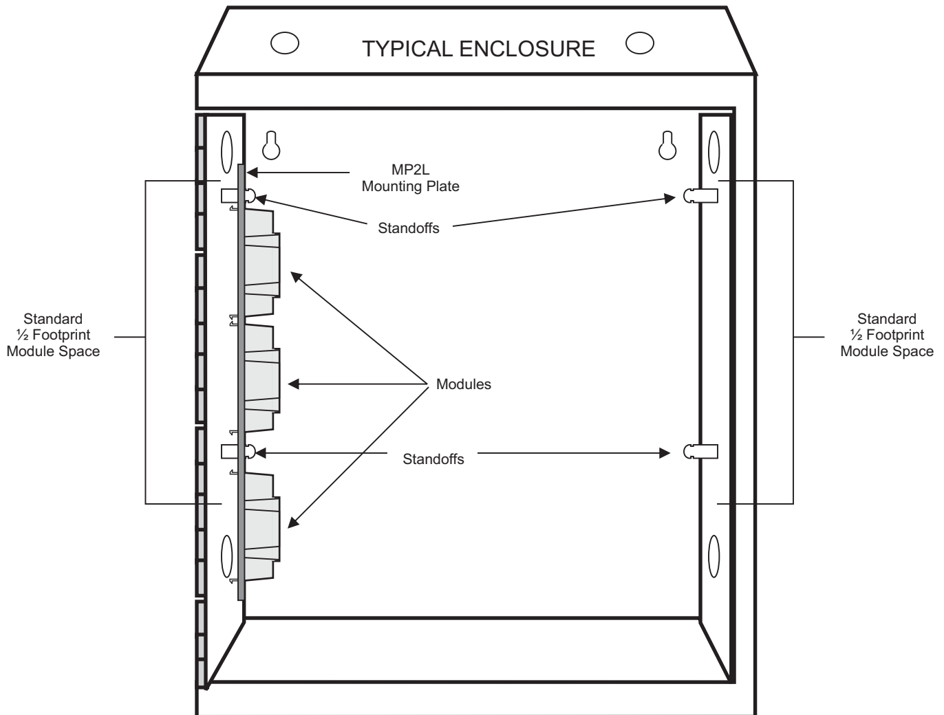
Figure 3, Mounting MP2L to Enclosure Standard 1/2 Footprint Module Space
